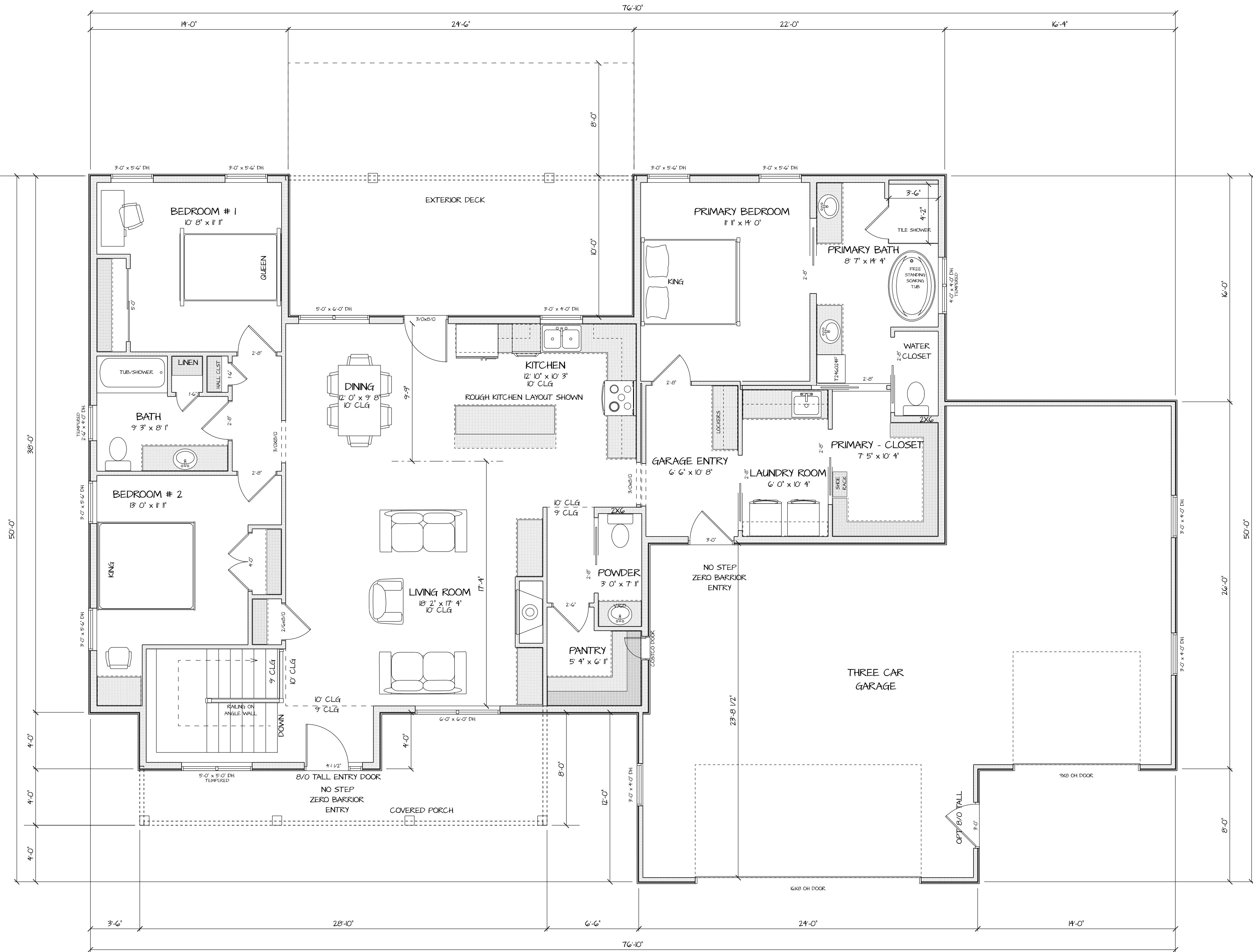
FIRST FLOOR SCALE: 1/4" = 1'-0"
